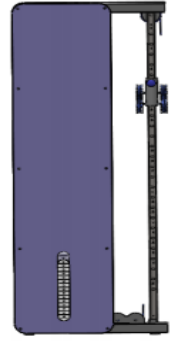
HOS-R004 Wall Mounted Pulley Weight:125kg Size(L*W*H) 780*2200*2220mm
